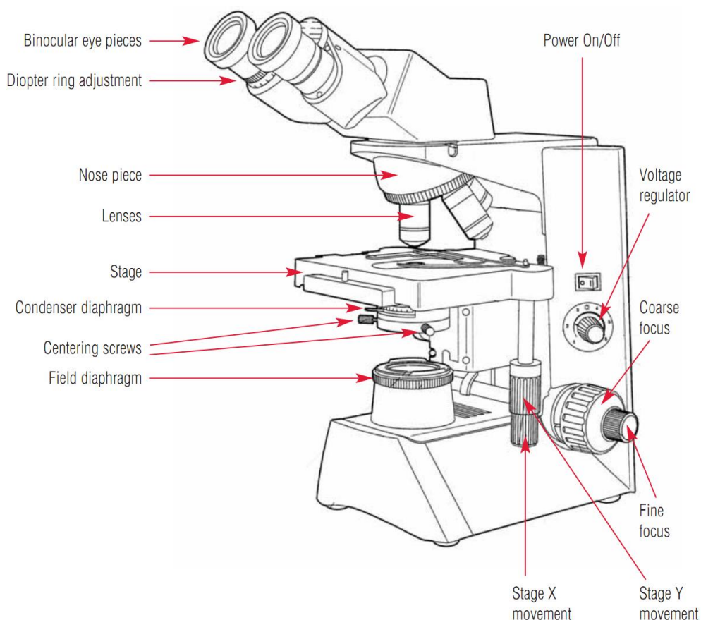
Figure 3. Microscope components
